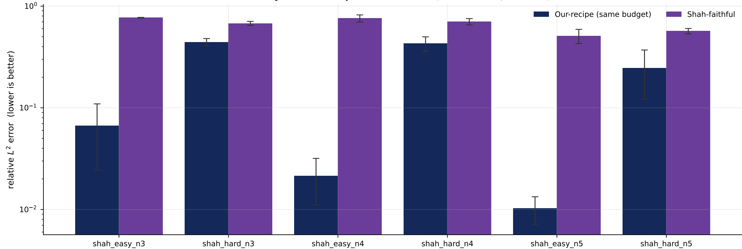
Accuracy at matched parameter count (mean \pm s.d., 3 seeds)
